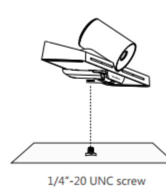
Mount on TV Stand or Tripod B
